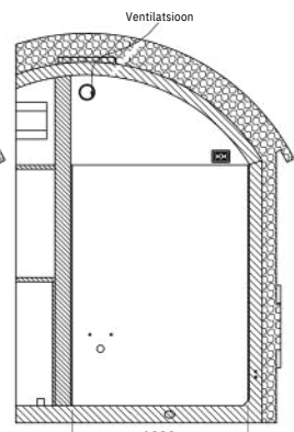
SECTION P-P
