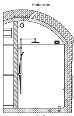
SECTION P-P
