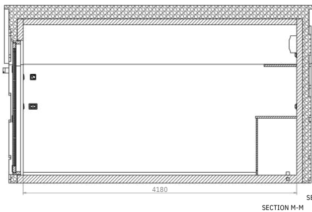
SECTION M-M
