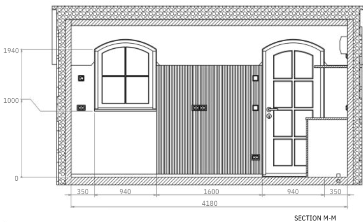
SECTION M-M
